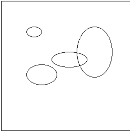
Figure 32: Synthetic contours
