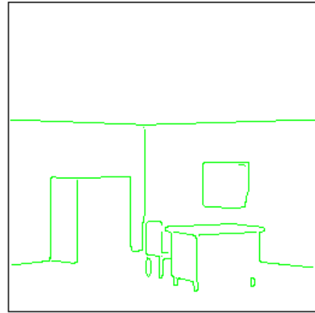
Figure 27: Contours
