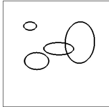
Figure 33: Ellipses detected
